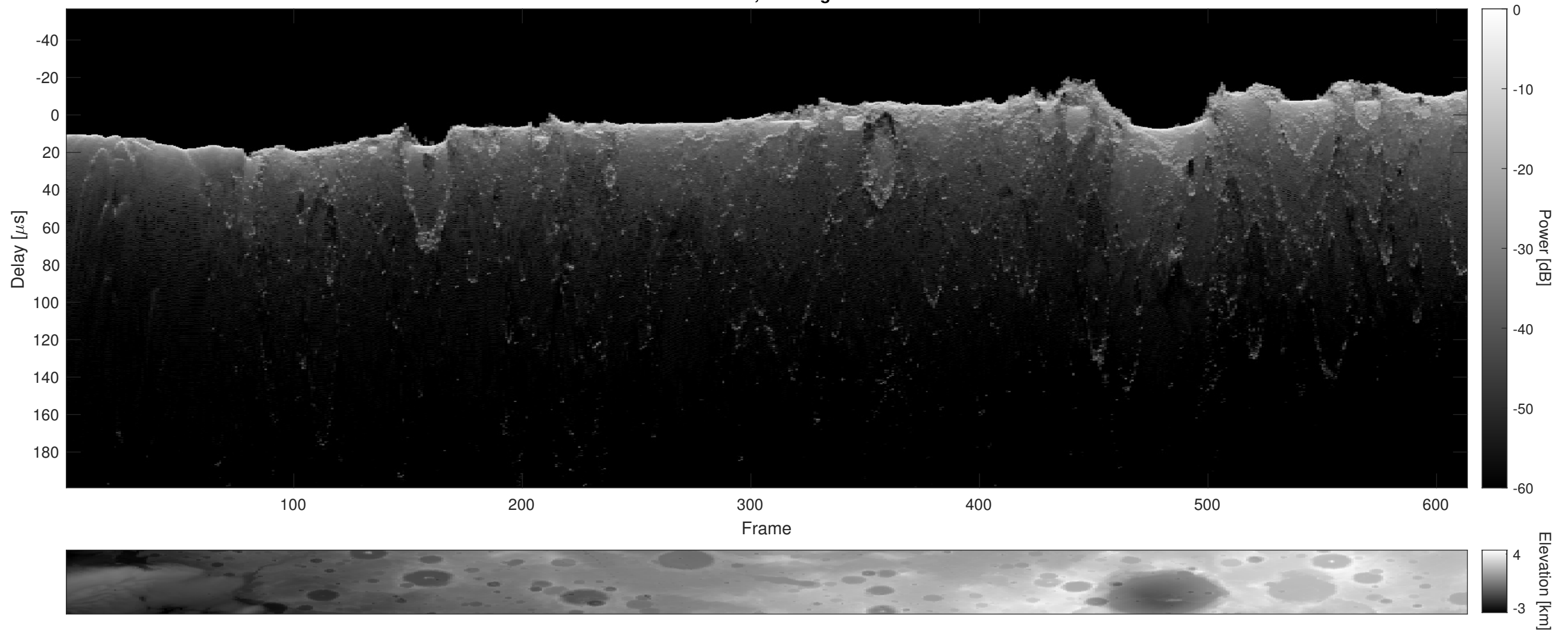
Orbit 3064, Cluttergram
