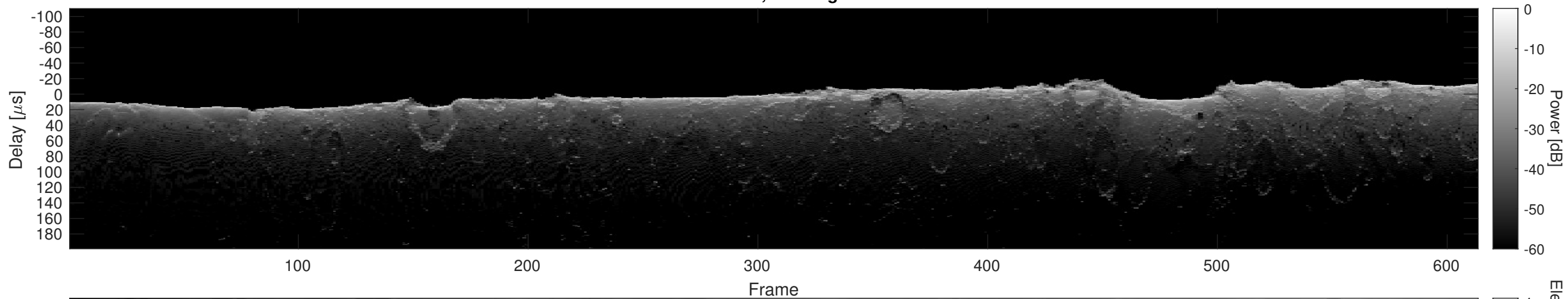
Orbit 3064, Cluttergram
