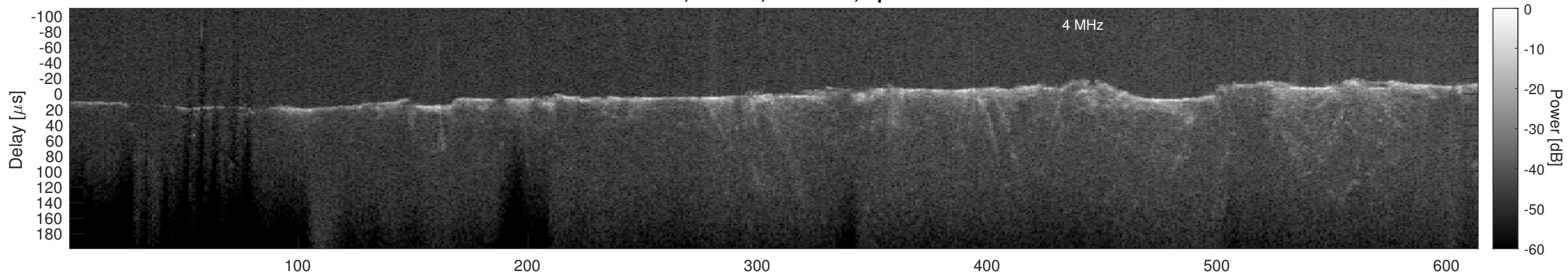
Orbit 3064, Cluttergram
