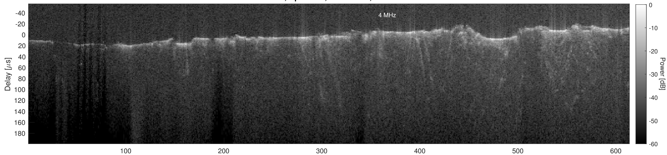
Orbit 3064, Cluttergram
