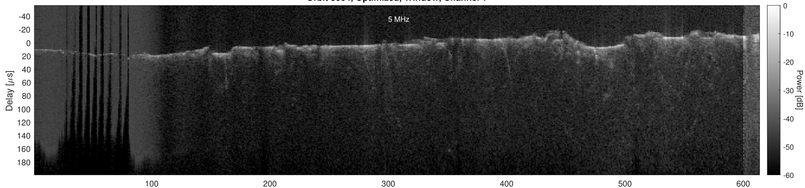
Orbit 3064, Optimized, Window, Channel 2
