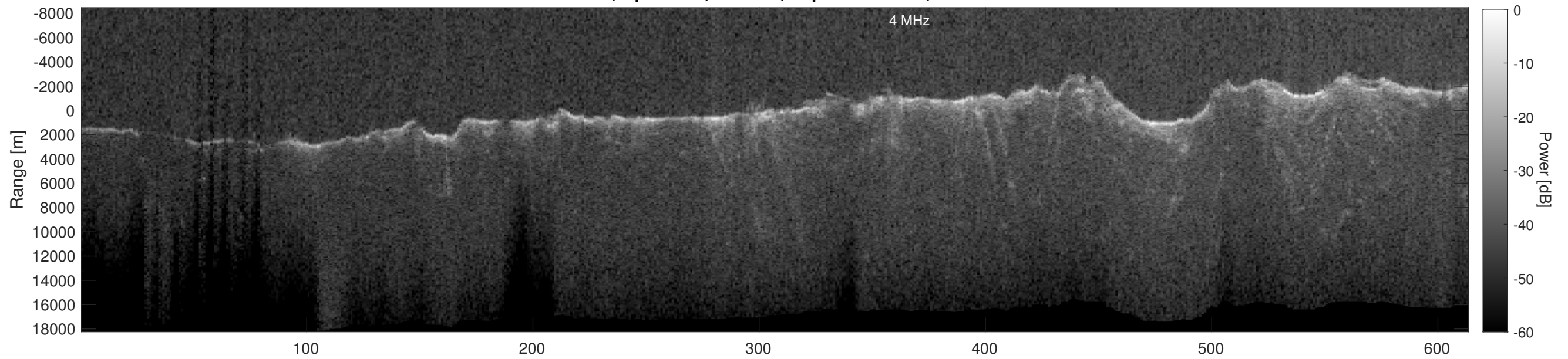
Orbit 3064, Depth-Corrected Cluttergram
