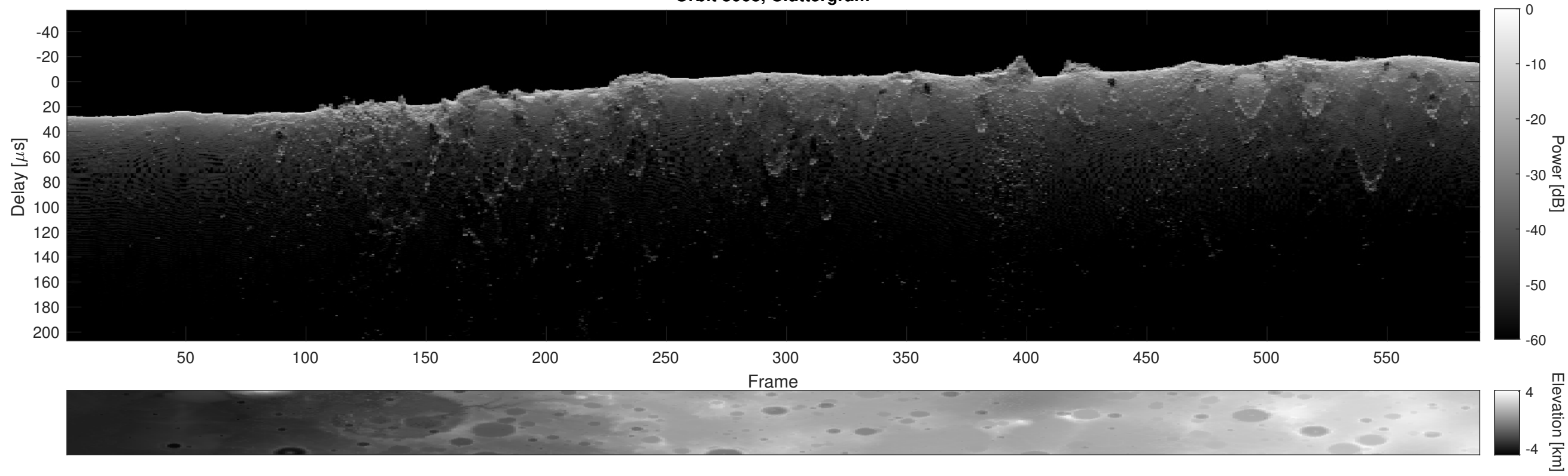
Orbit 3068, Cluttergram
