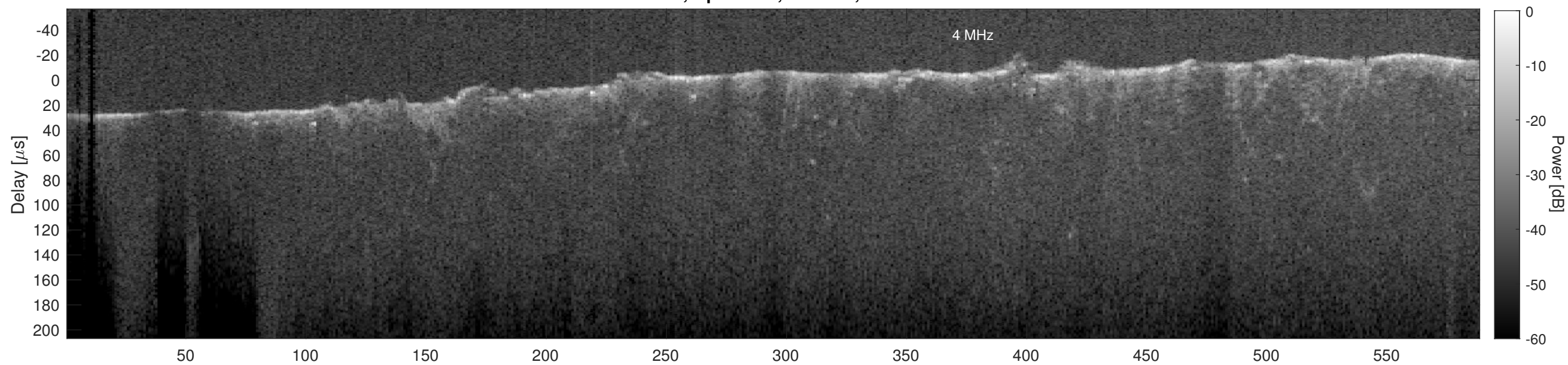
Orbit 3068, Cluttergram
