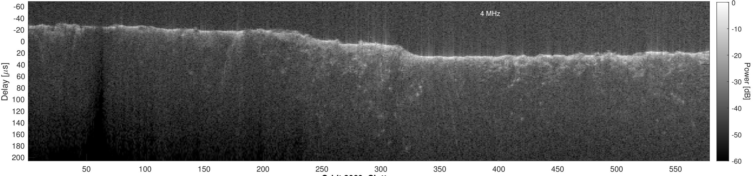
Orbit 3069, Cluttergram
