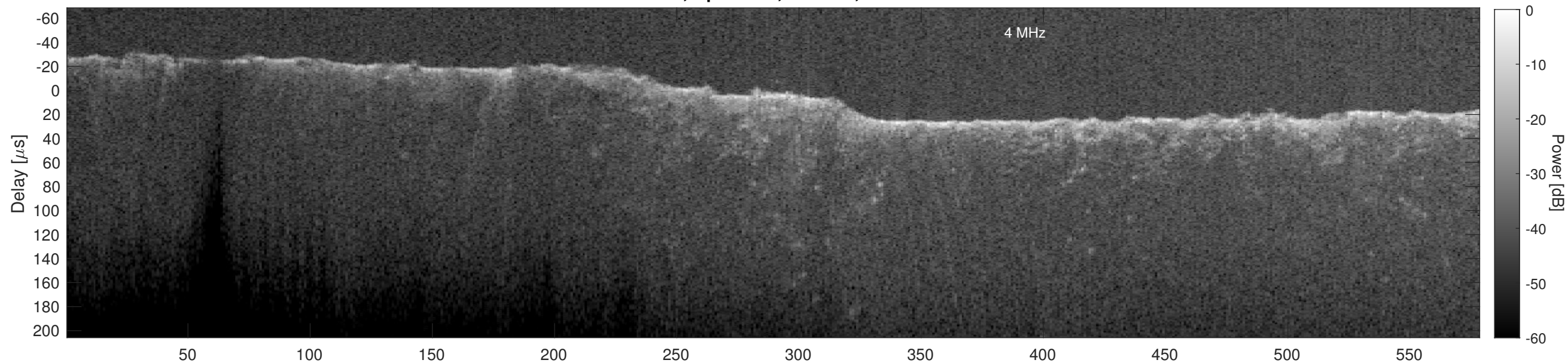
Orbit 3069, Cluttergram
