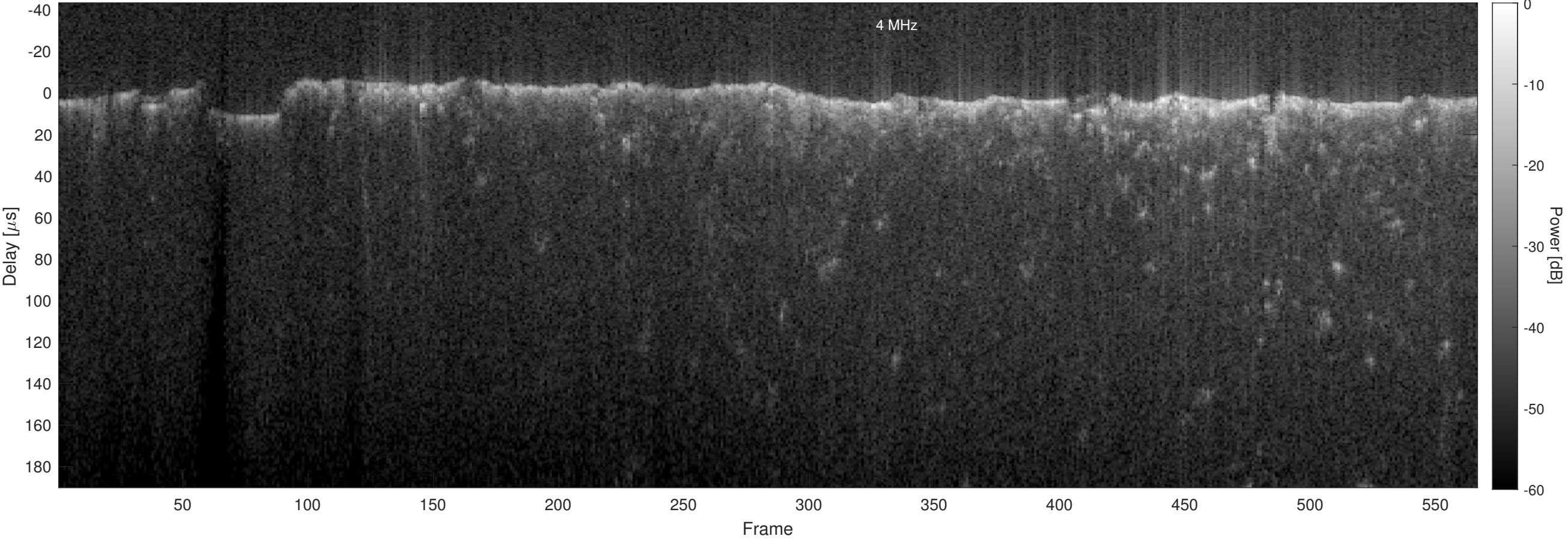
Orbit 3073, Optimized, No Window, Channel 2
