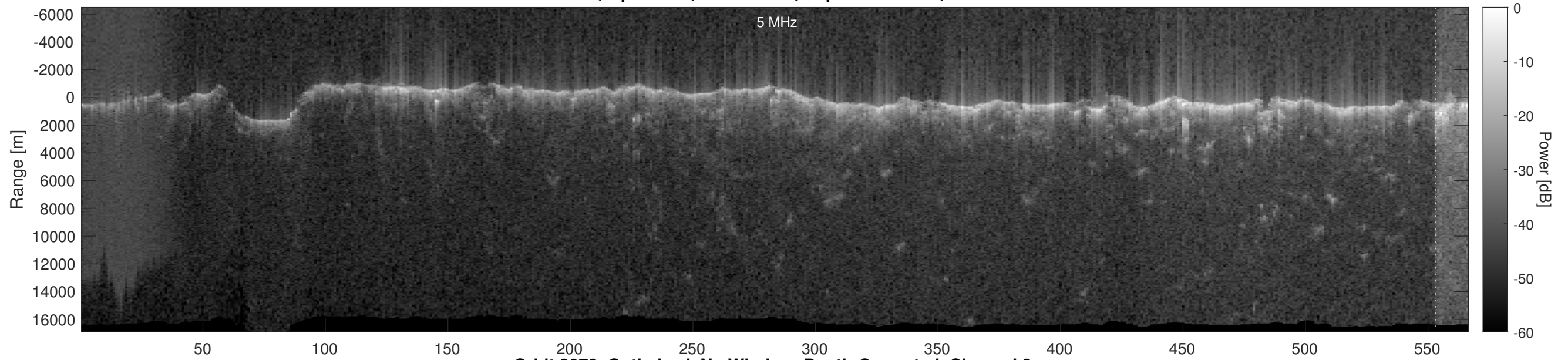
Orbit 3073, Optimized, No Window, Depth-Corrected, Channel 2
