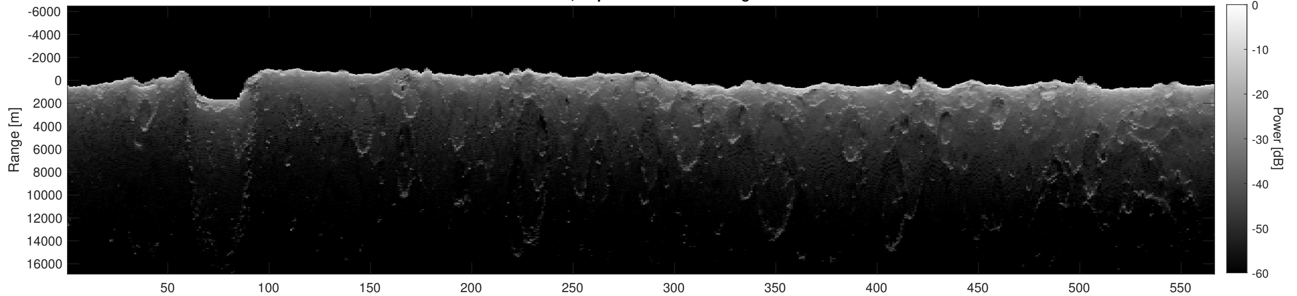
Orbit 3073, Depth-Corrected Cluttergram
