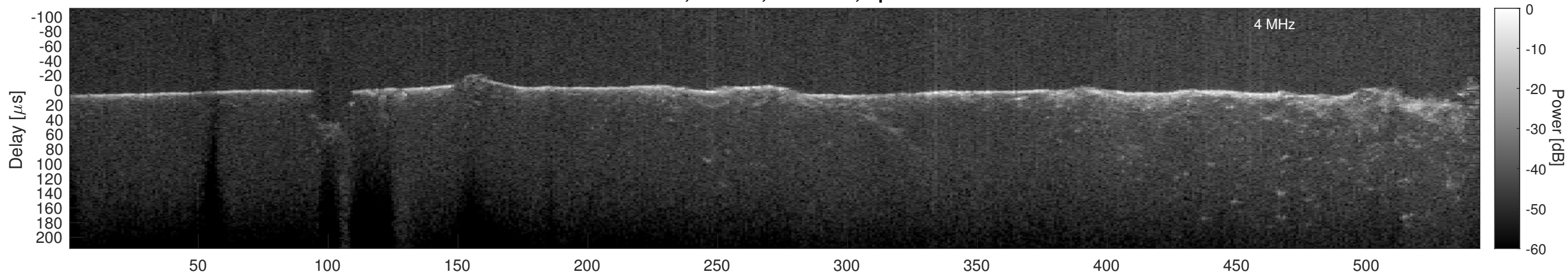
Orbit 3074, Cluttergram
