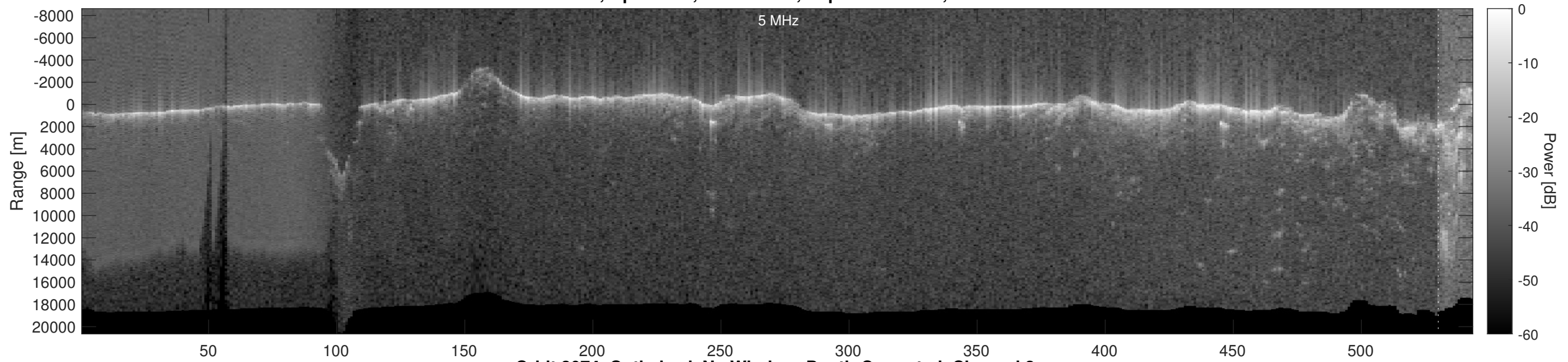
Orbit 3074, Optimized, No Window, Depth-Corrected, Channel 2
