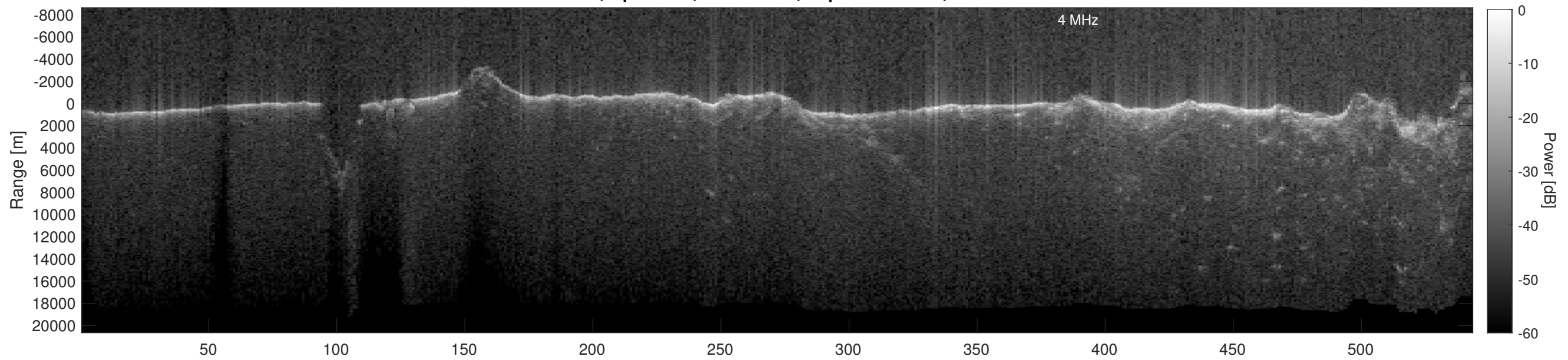
Orbit 3074, Depth-Corrected Cluttergram
