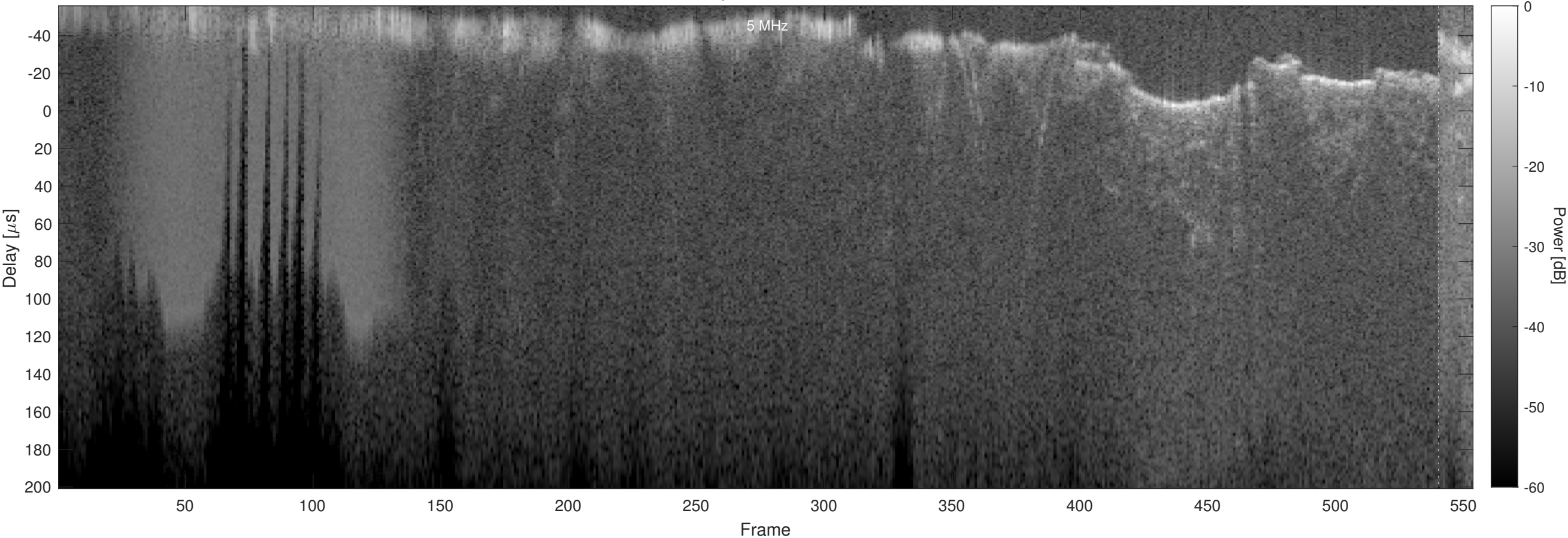
Orbit 3075, Chapman, Window, Channel 2
