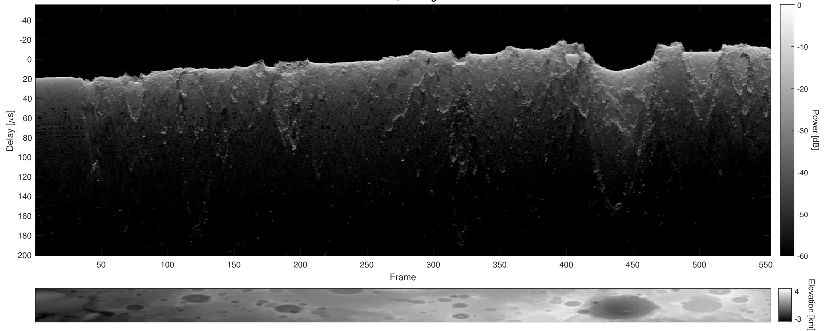
Orbit 3075, Cluttergram
