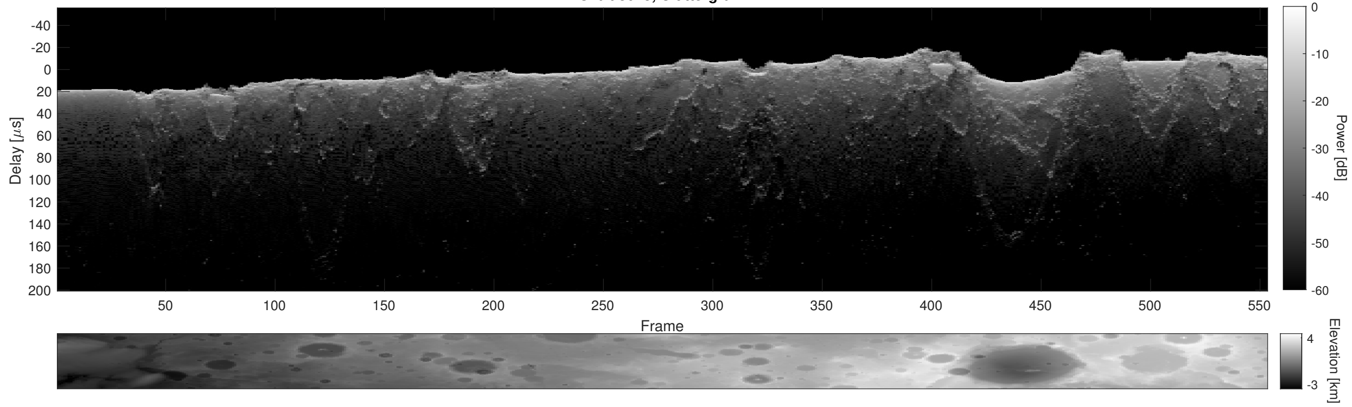
Orbit 3075, Cluttergram
