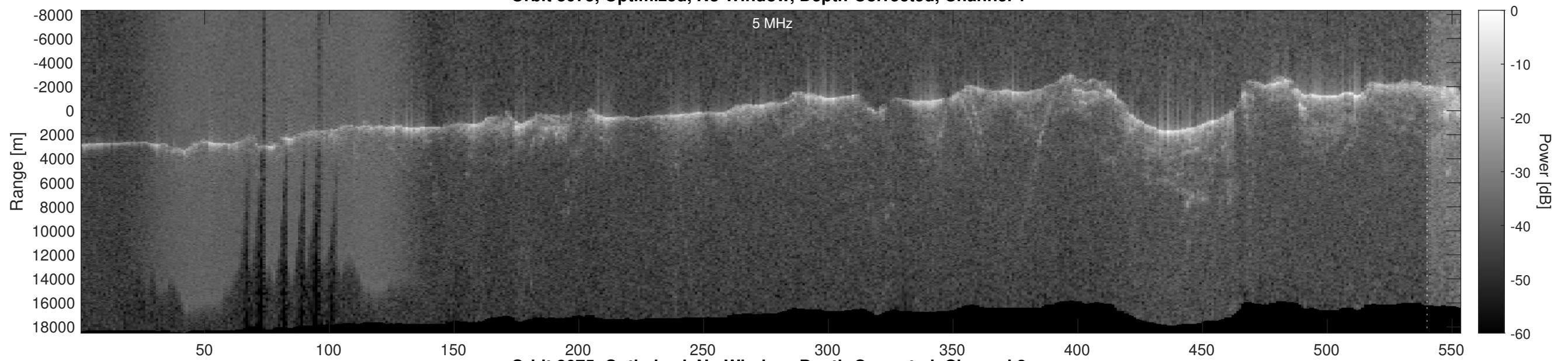
Orbit 3075, Optimized, No Window, Depth-Corrected, Channel 2
