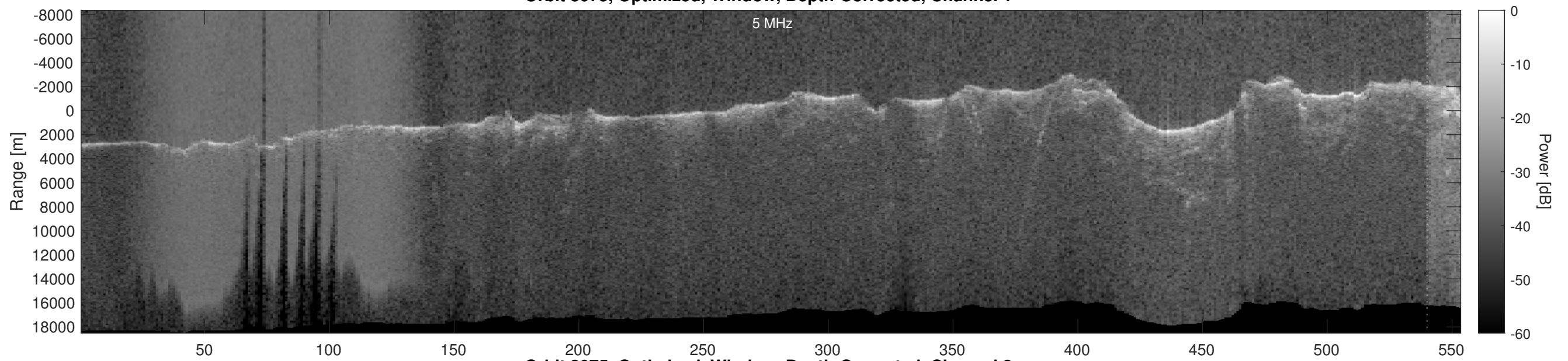
Orbit 3075, Optimized, Window, Depth-Corrected, Channel 2
