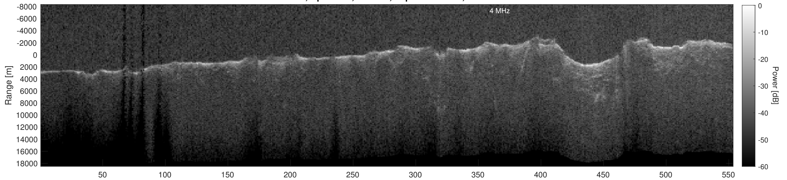
Orbit 3075, Depth-Corrected Cluttergram
