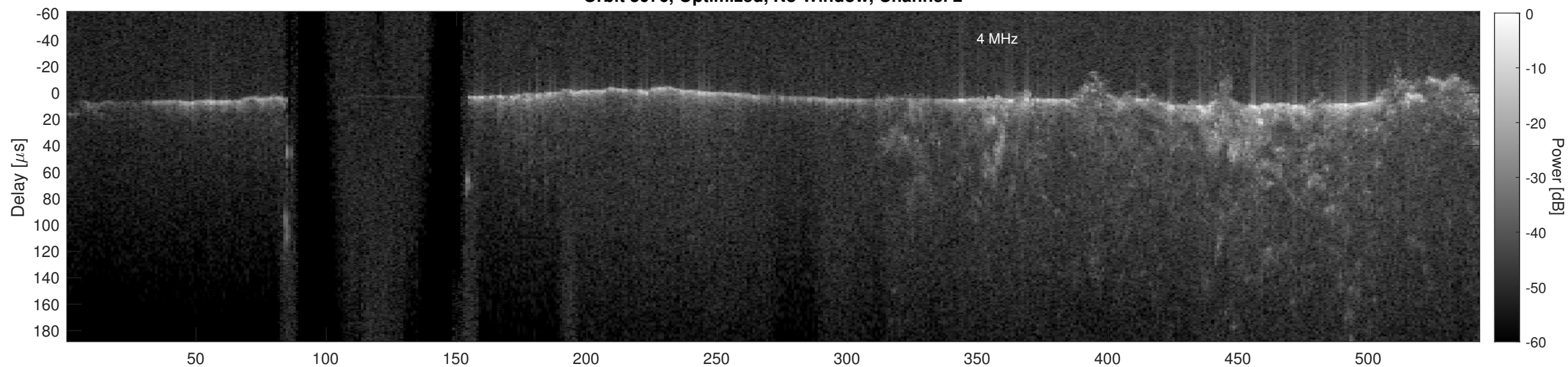
Orbit 3076, Cluttergram
