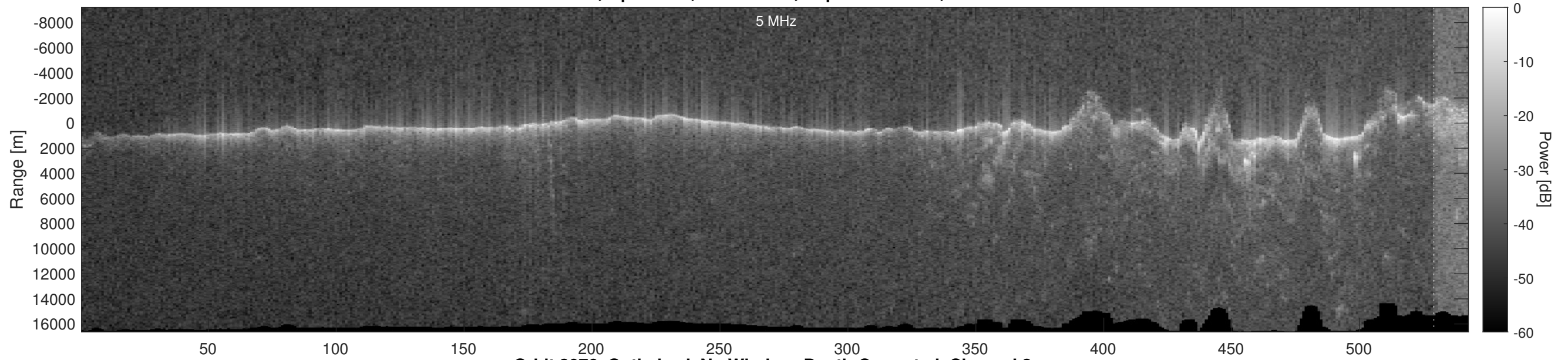
Orbit 3076, Optimized, No Window, Depth-Corrected, Channel 2
