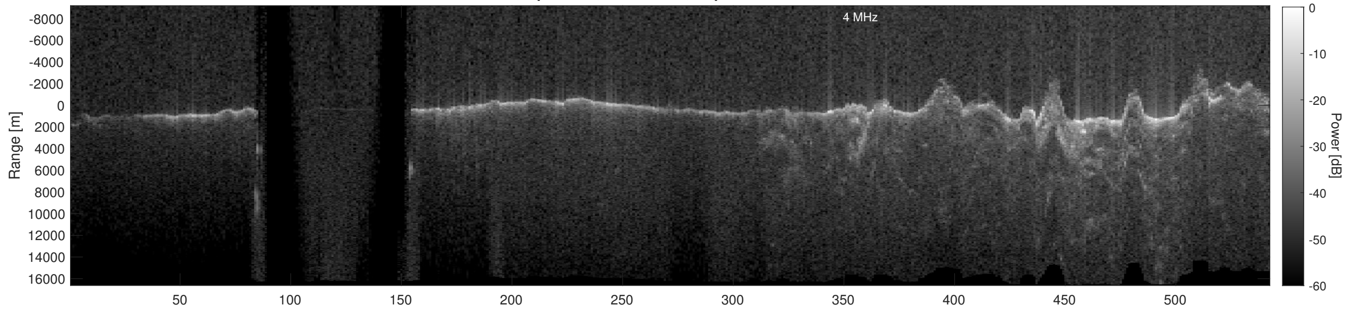
Orbit 3076, Depth-Corrected Cluttergram
