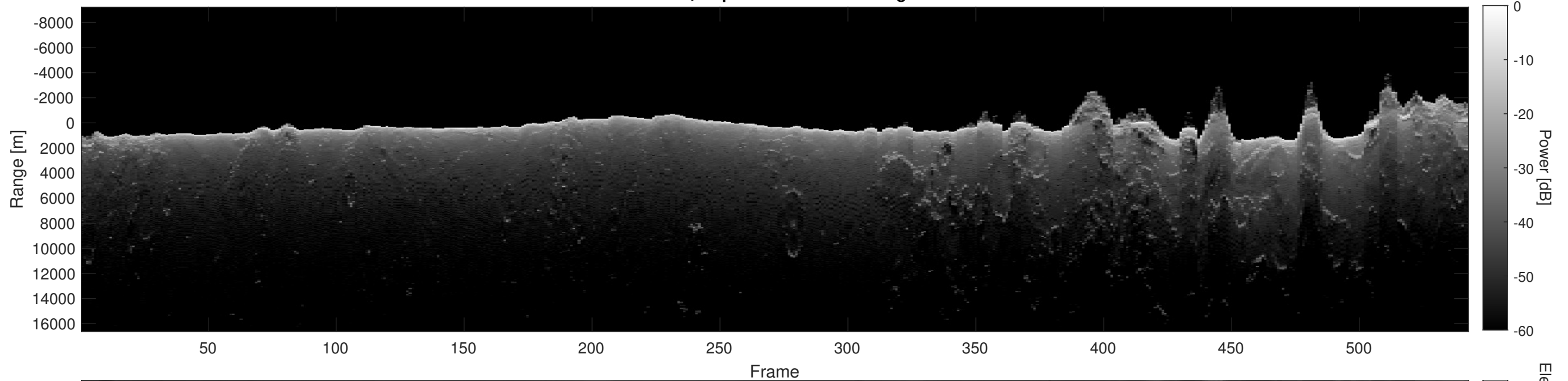
Orbit 3076, Depth-Corrected Cluttergram
