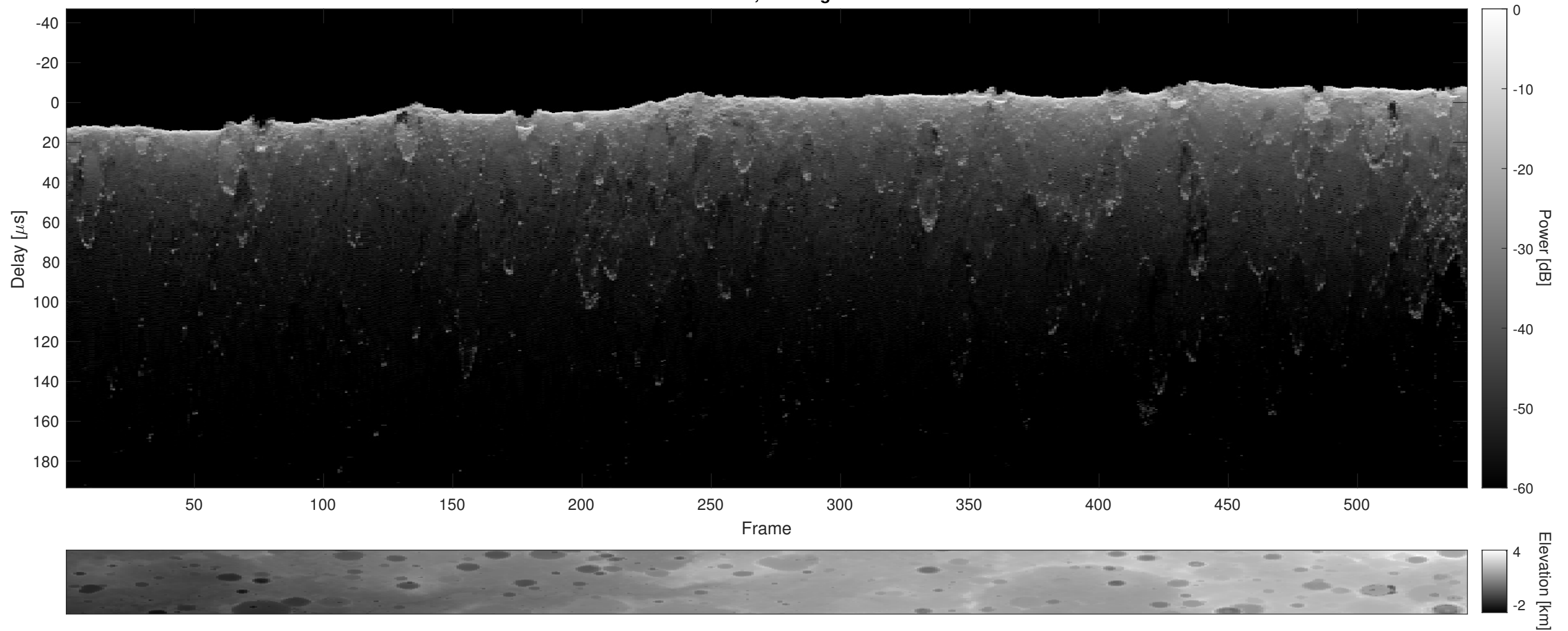
Orbit 3077, Cluttergram
