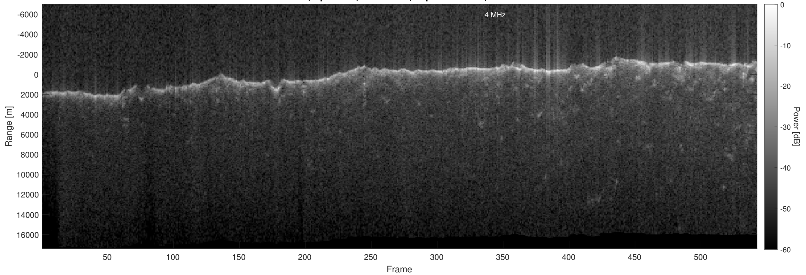
Orbit 3077, Optimized, No Window, Depth-Corrected, Channel 2
