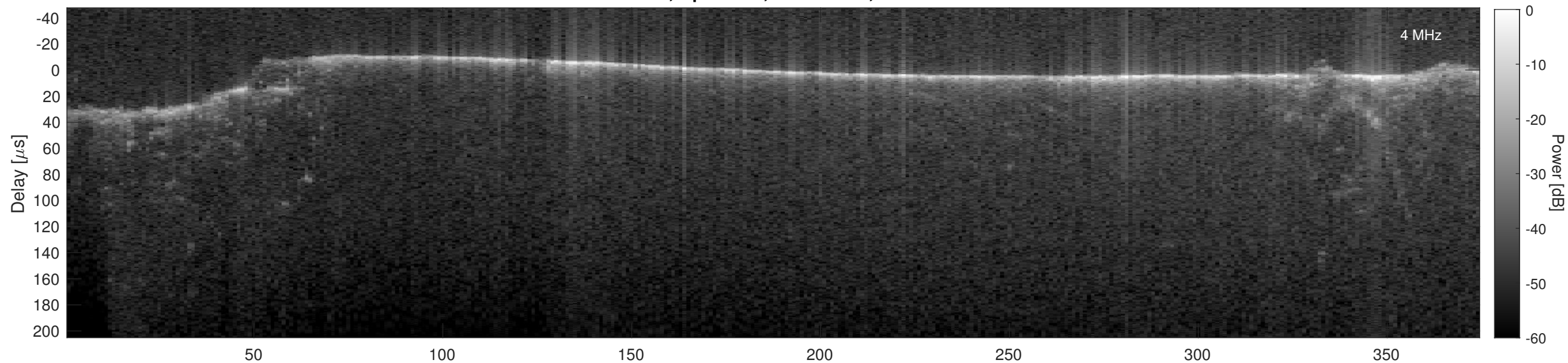
Orbit 3078, Cluttergram
