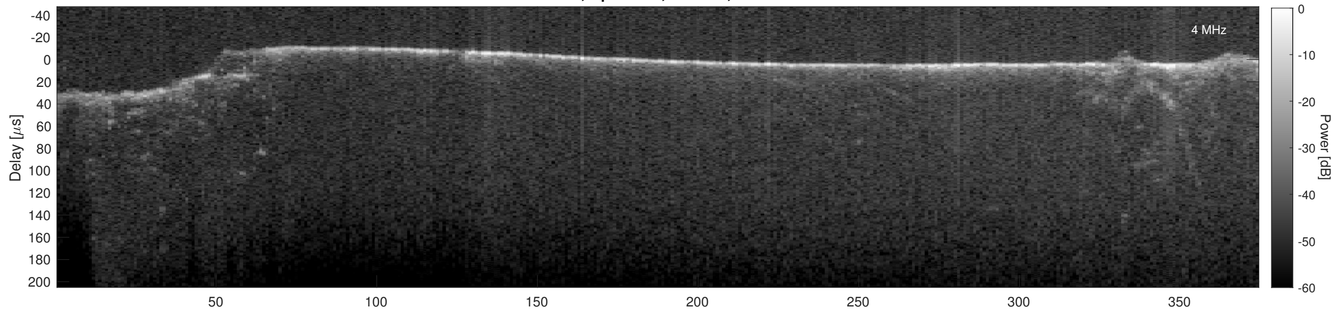
Orbit 3078, Cluttergram
