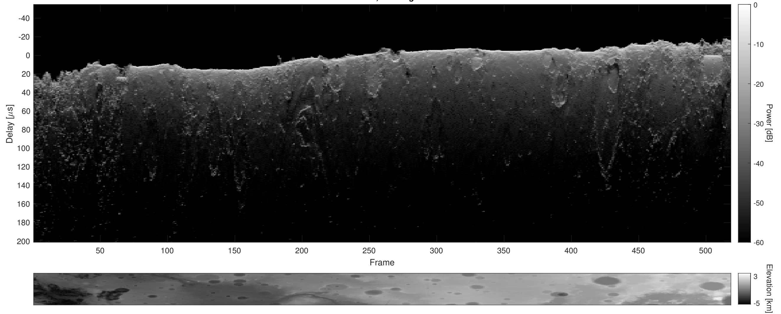
Orbit 3081, Cluttergram
