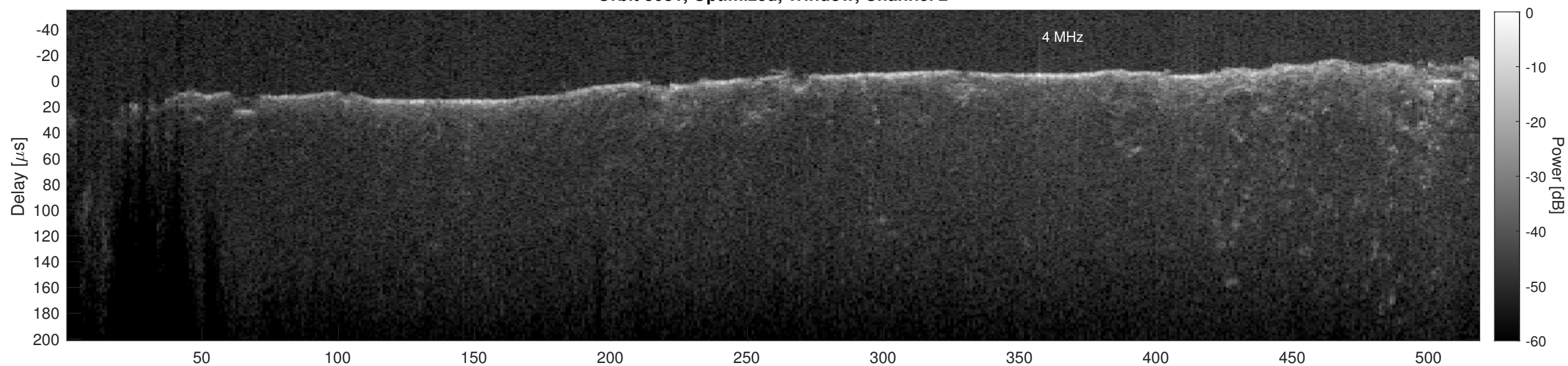
Orbit 3081, Cluttergram
