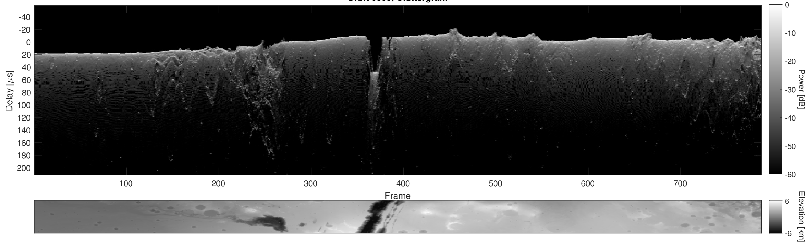
Orbit 3085, Cluttergram
