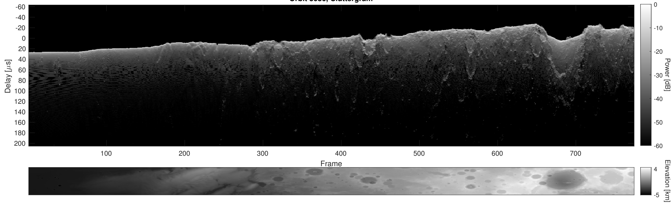
Orbit 3086, Cluttergram
