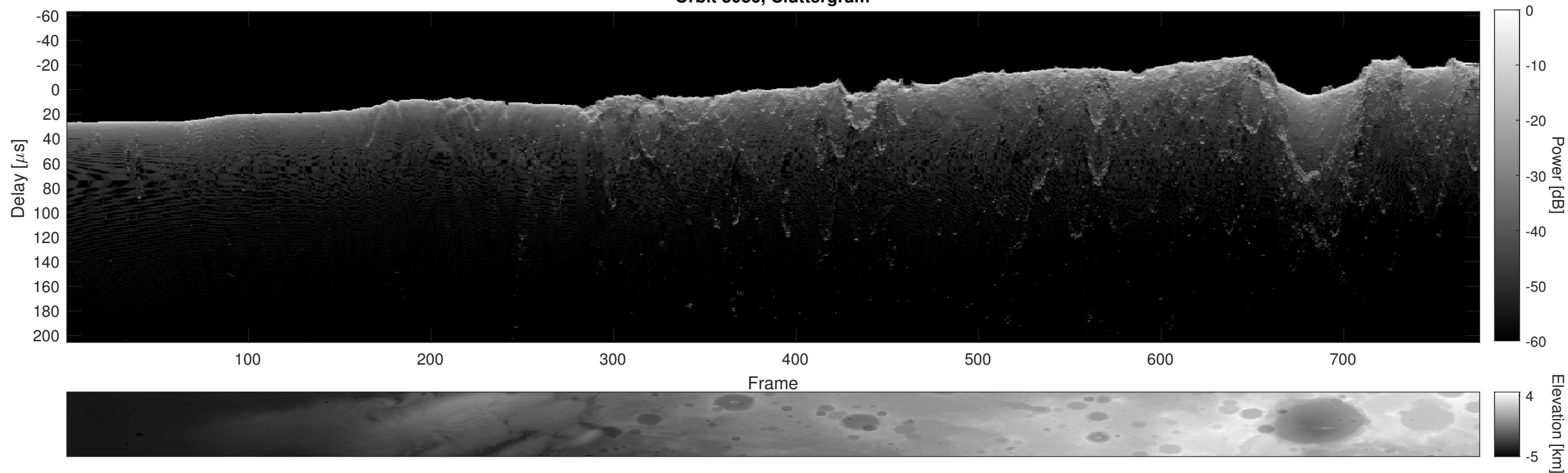
Orbit 3086, Cluttergram
