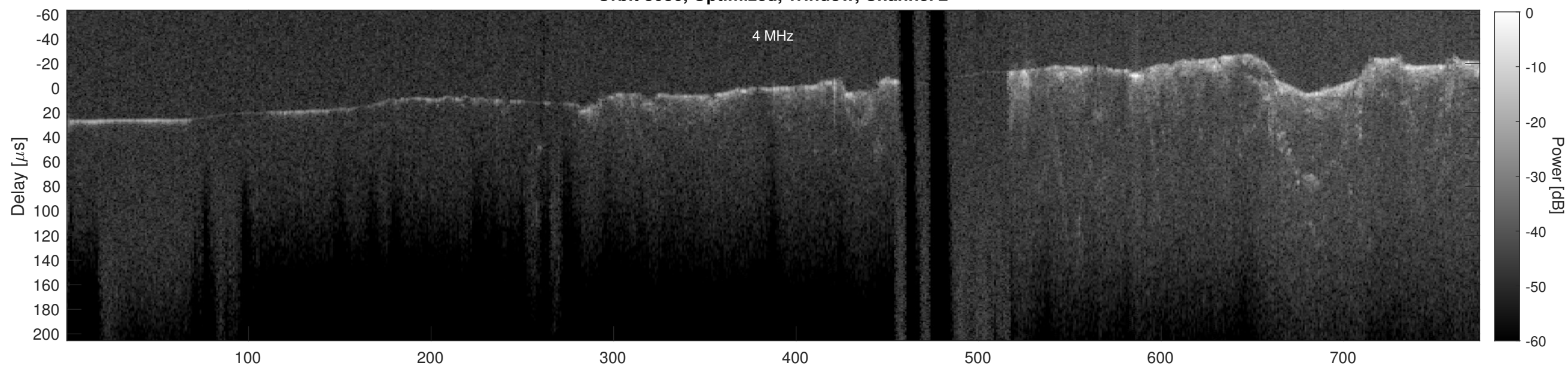
Orbit 3086, Cluttergram
