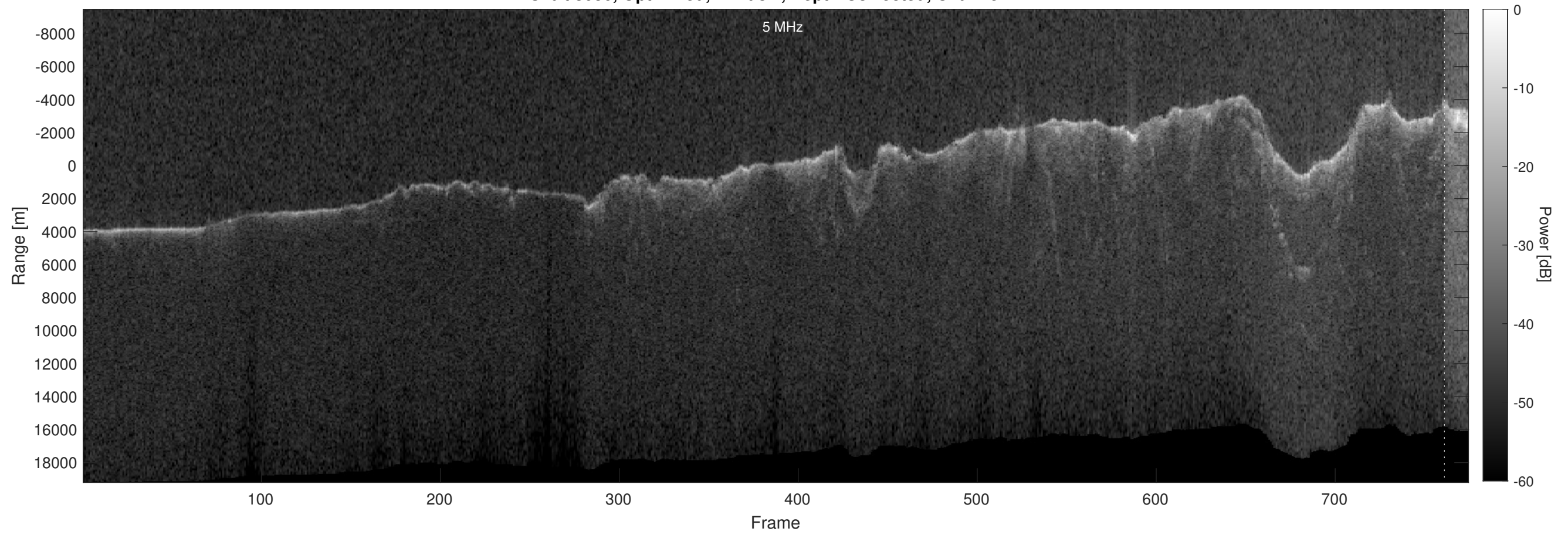
Orbit 3086, Optimized, Window, Depth-Corrected, Channel 2
