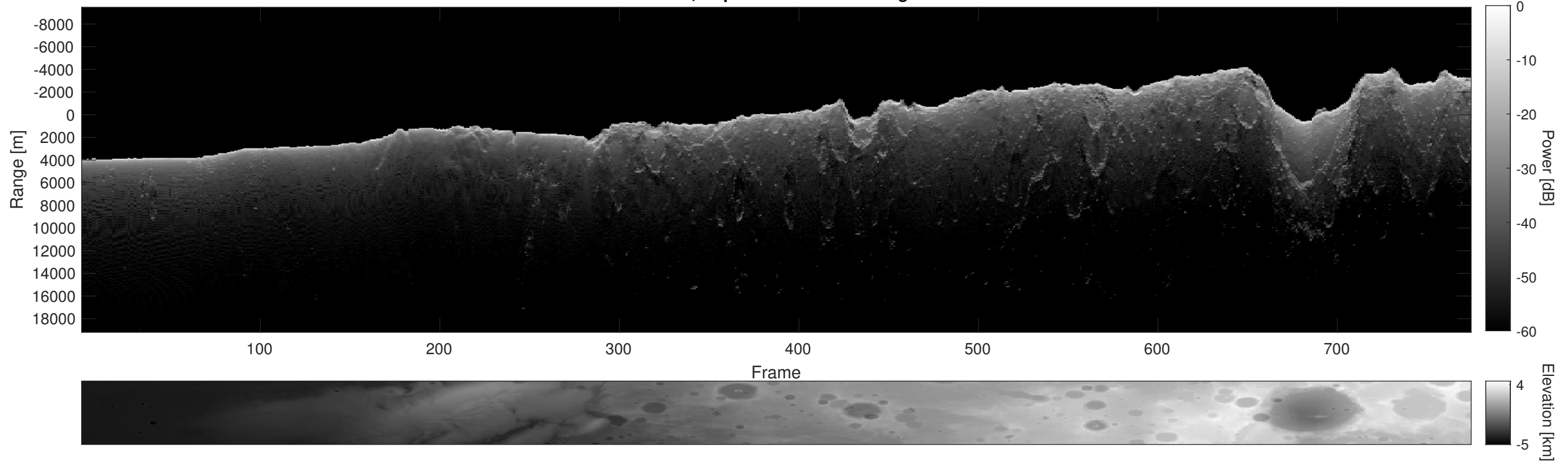
Orbit 3086, Depth-Corrected Cluttergram
