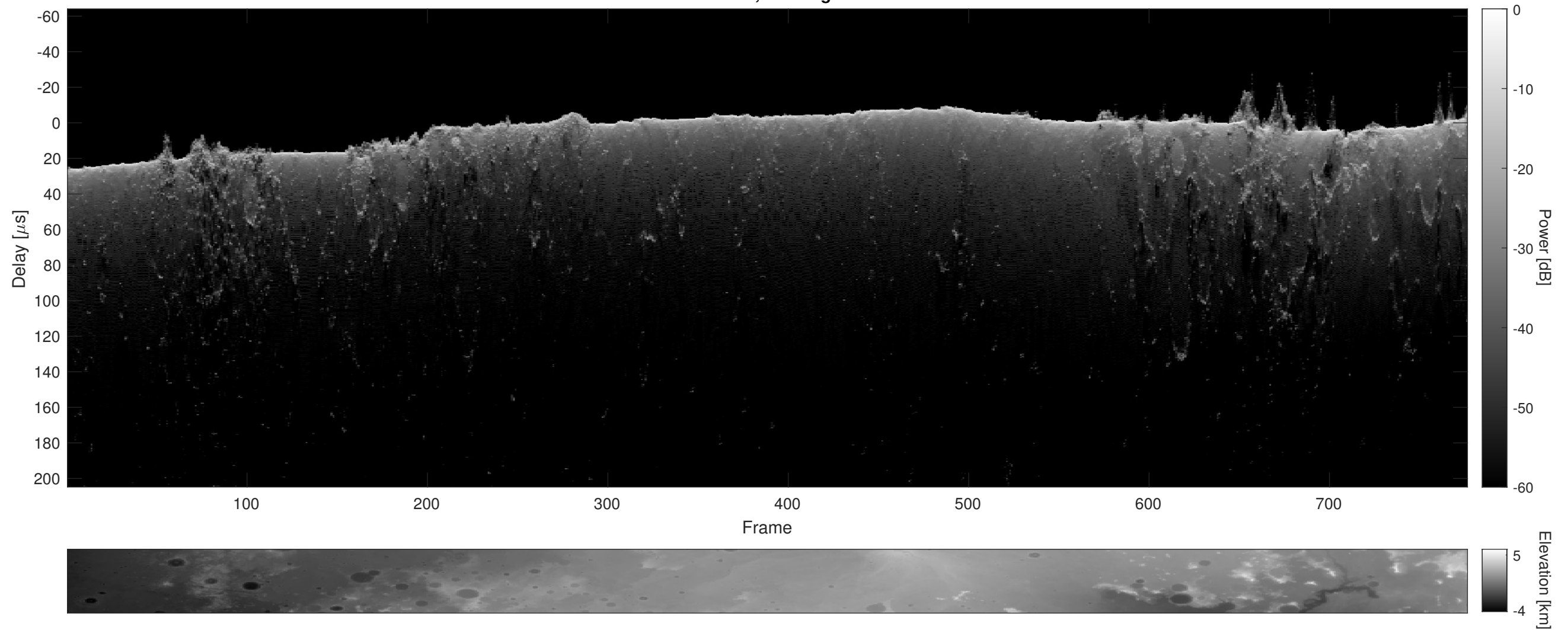
Orbit 3087, Cluttergram
