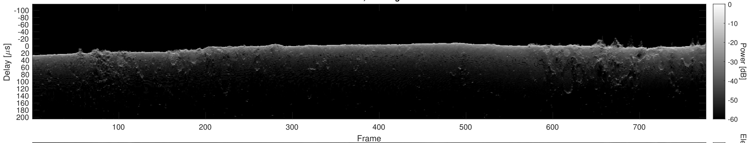
Orbit 3087, Cluttergram
