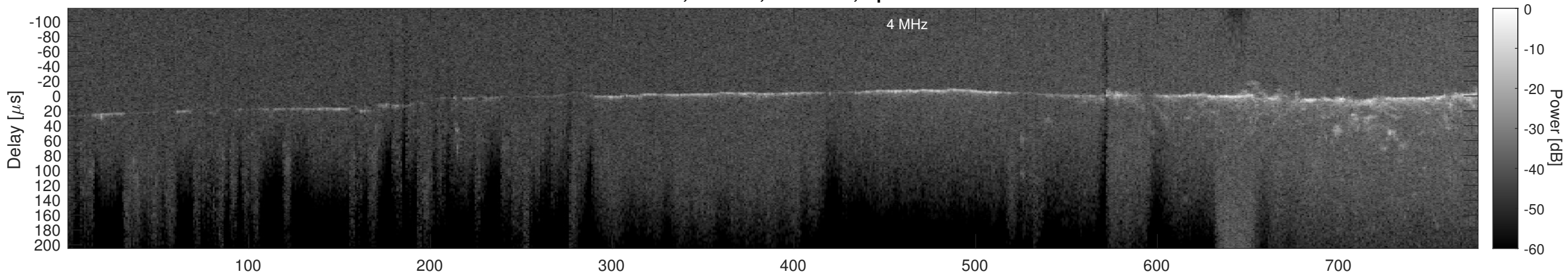
Orbit 3087, Cluttergram
