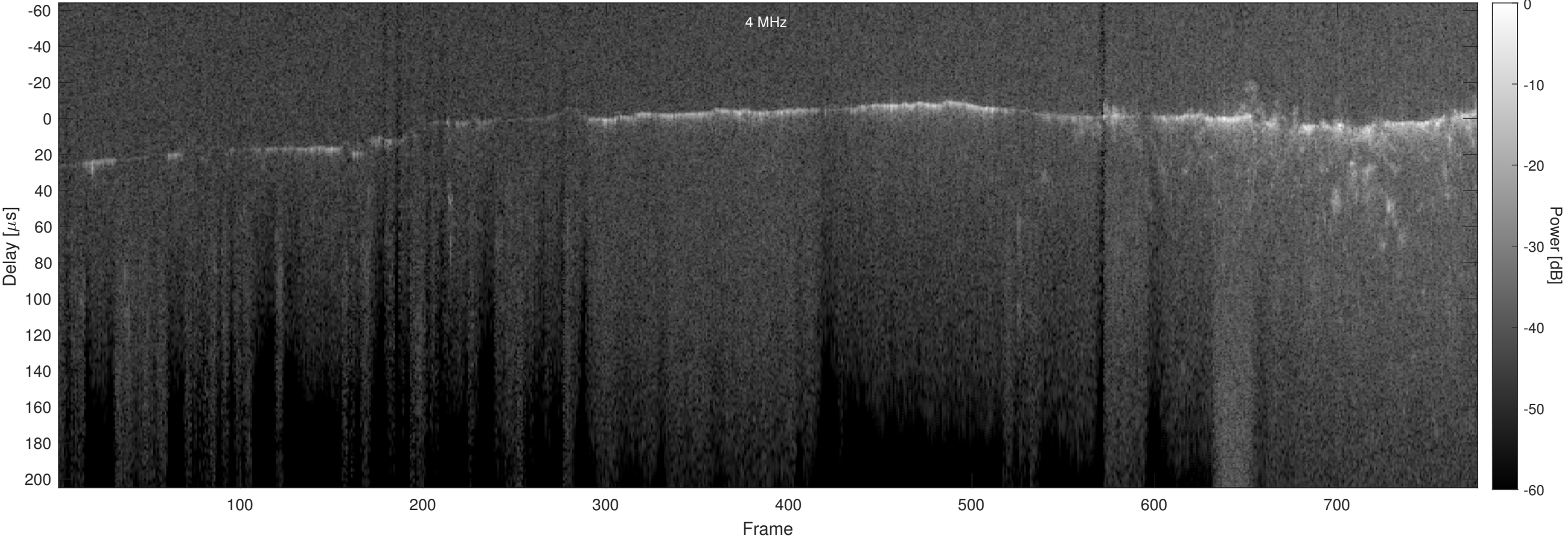
Orbit 3087, Optimized, No Window, Channel 2
