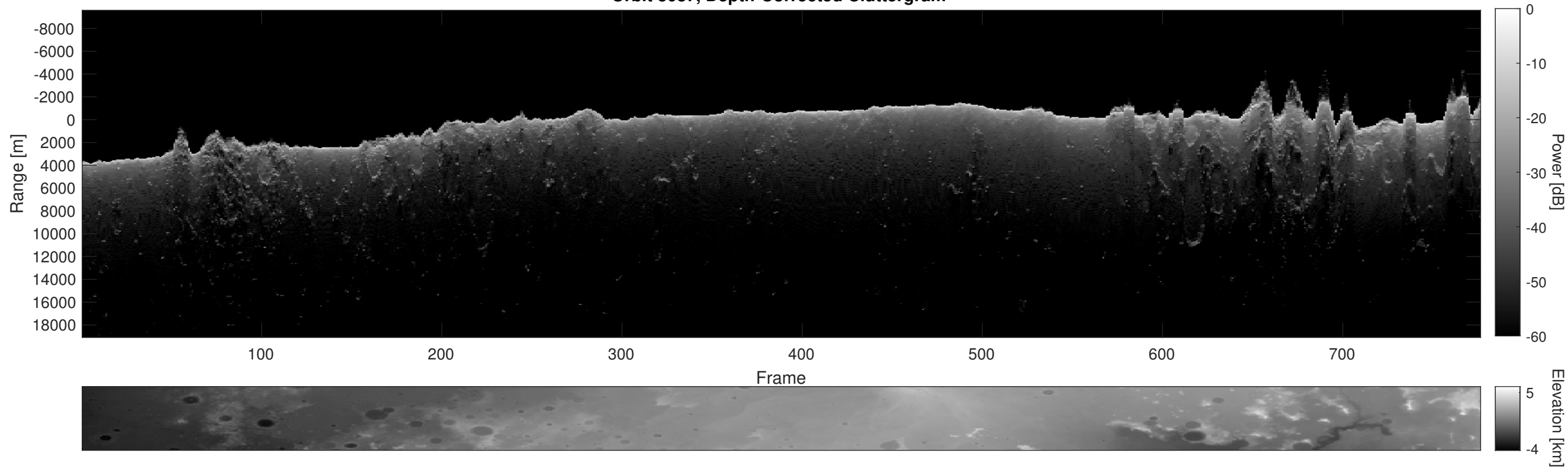
Orbit 3087, Depth-Corrected Cluttergram
