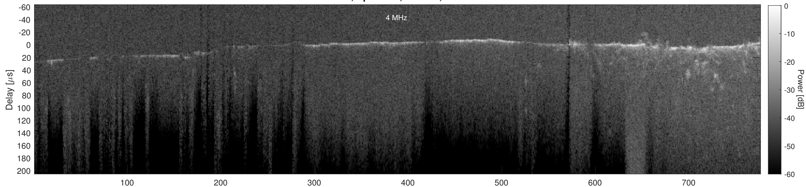
Orbit 3087, Cluttergram
