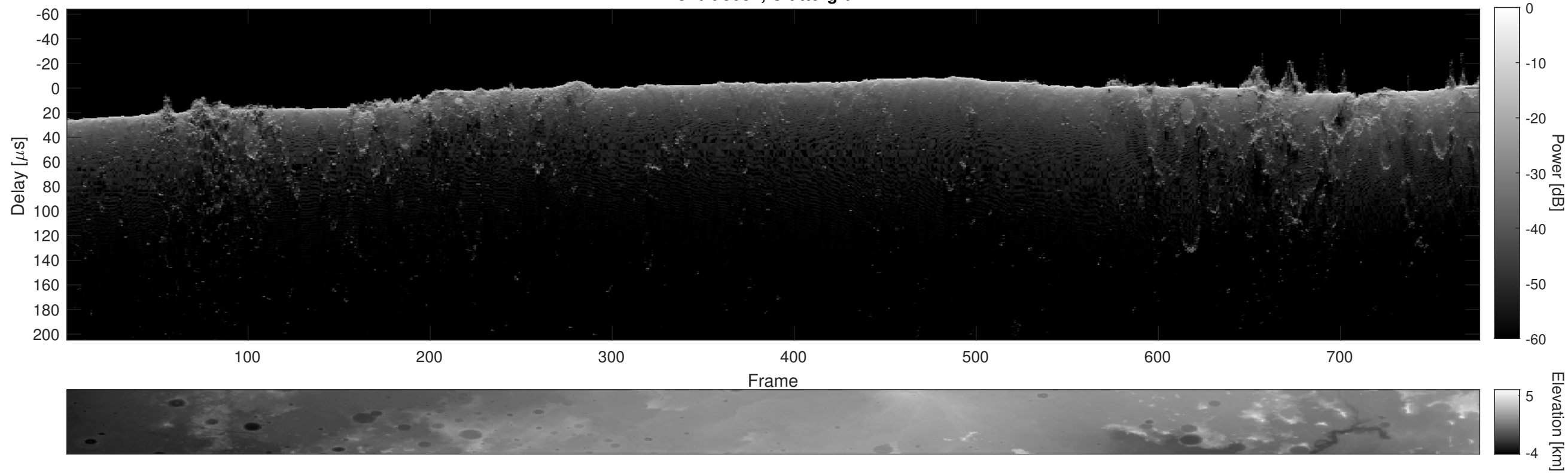
Orbit 3087, Cluttergram
