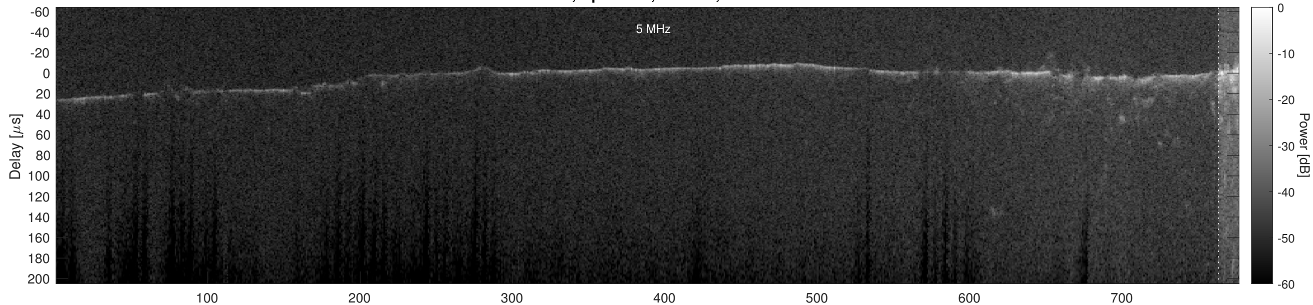
Orbit 3087, Optimized, Window, Channel 2
