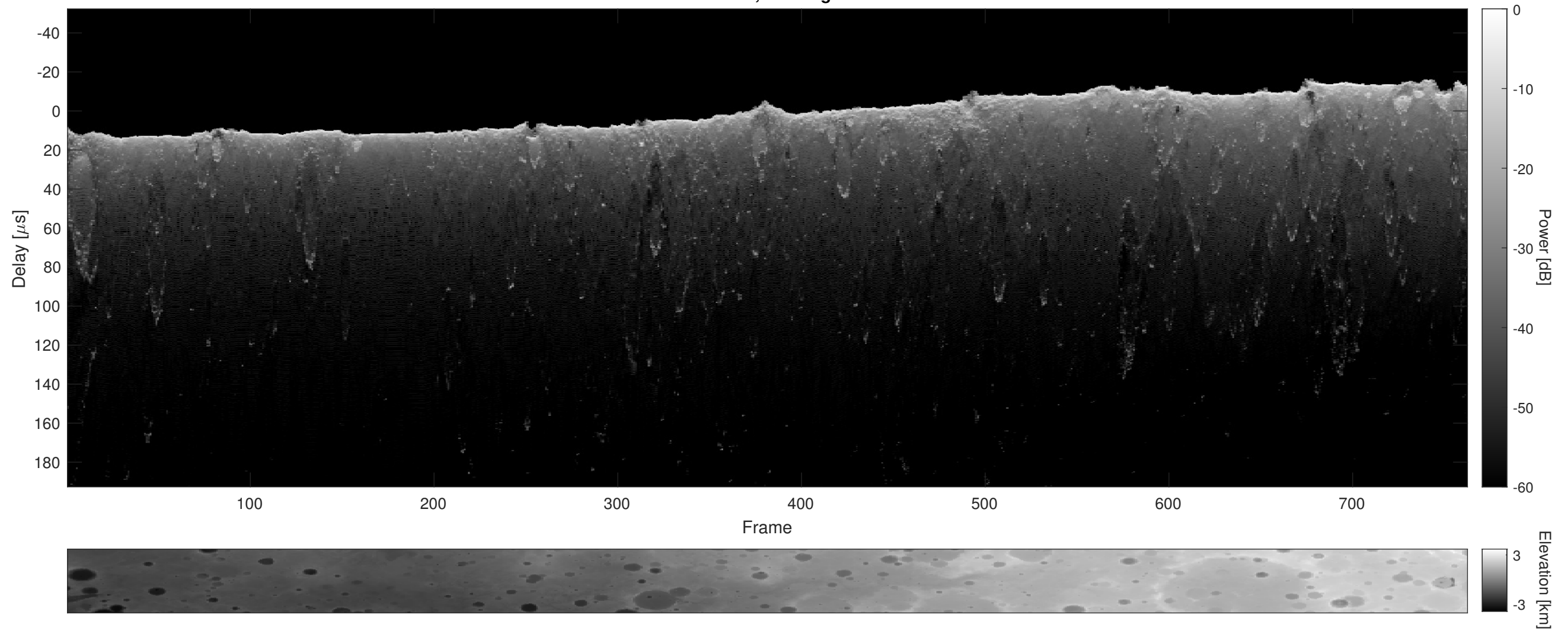
Orbit 3088, Cluttergram
