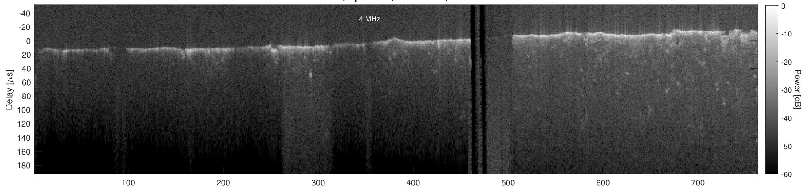
Orbit 3088, Cluttergram
