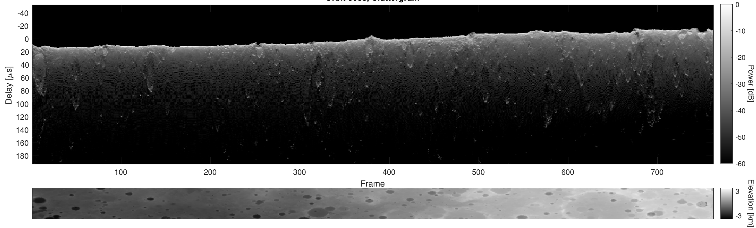
Orbit 3088, Cluttergram
