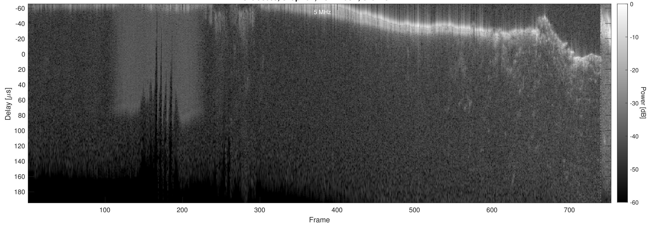
Orbit 3089, Chapman, No Window, Channel 2
