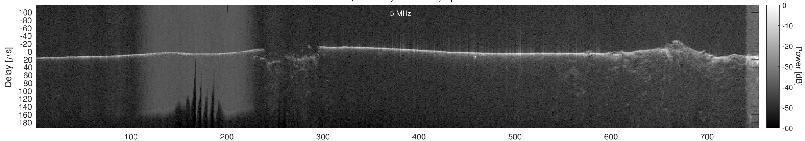
Orbit 3089, Cluttergram
