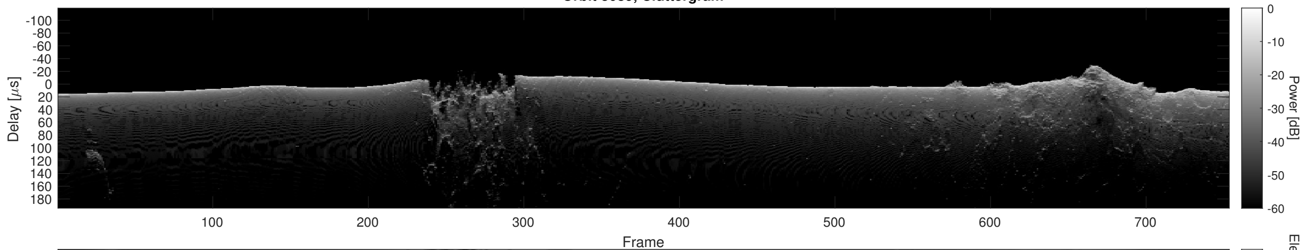
Orbit 3089, Cluttergram
