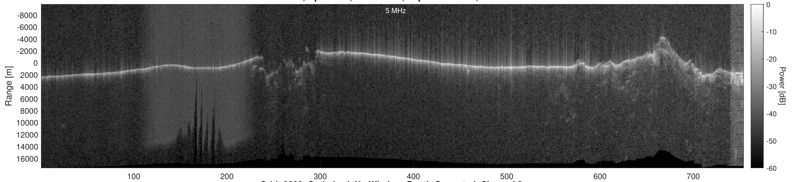
Orbit 3089, Optimized, No Window, Depth-Corrected, Channel 2
