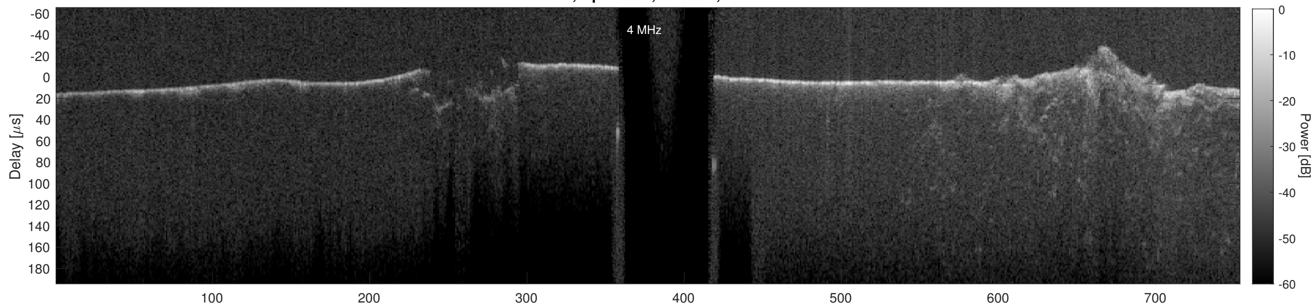
Orbit 3089, Cluttergram
