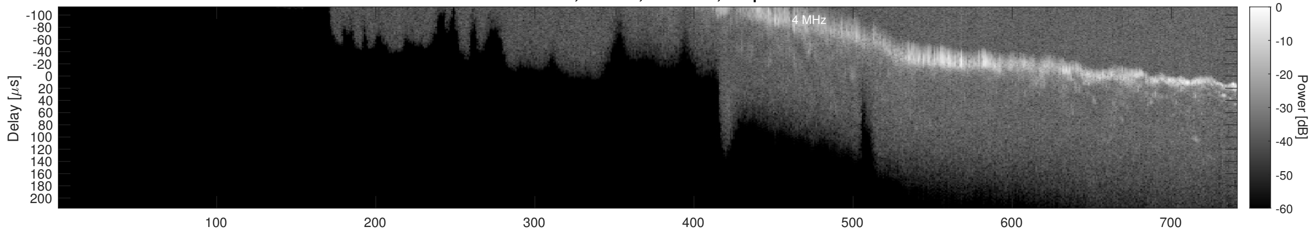
Orbit 3091, Window, Channel 2, Optimized
