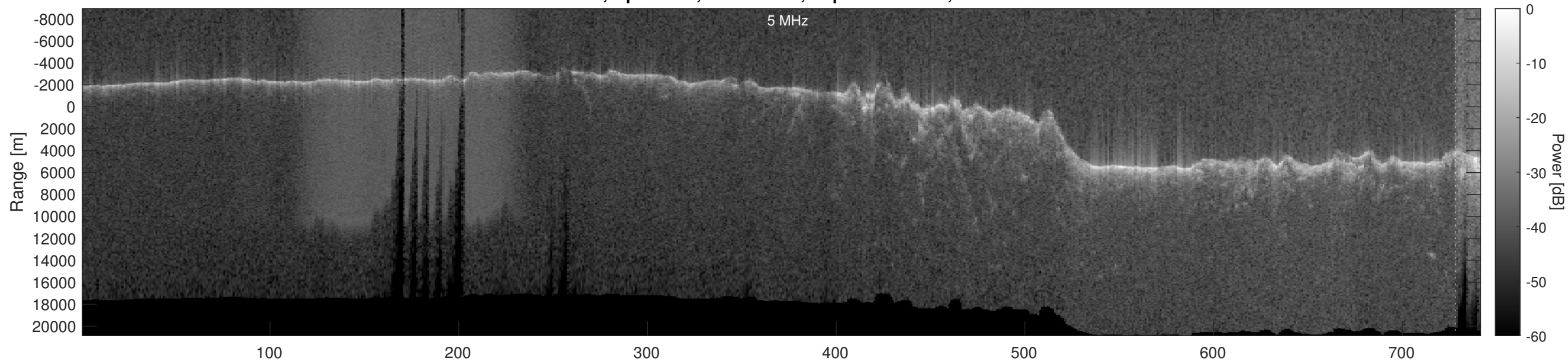
Orbit 3091, Optimized, No Window, Depth-Corrected, Channel 2
