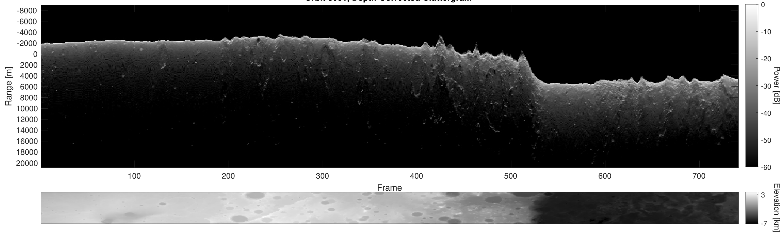
Orbit 3091, Depth-Corrected Cluttergram
