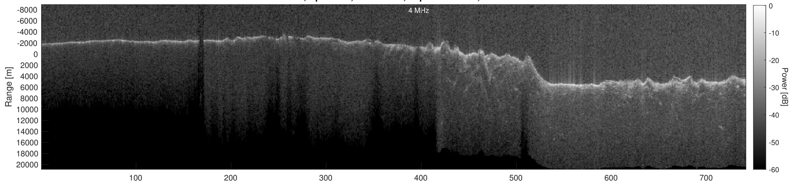
Orbit 3091, Depth-Corrected Cluttergram
