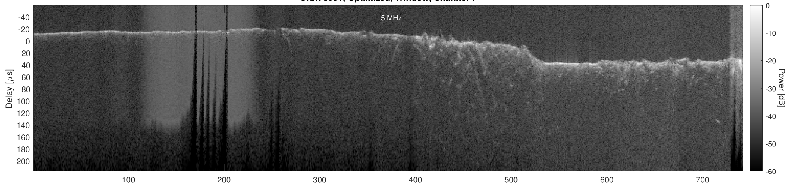
Orbit 3091, Optimized, Window, Channel 2
