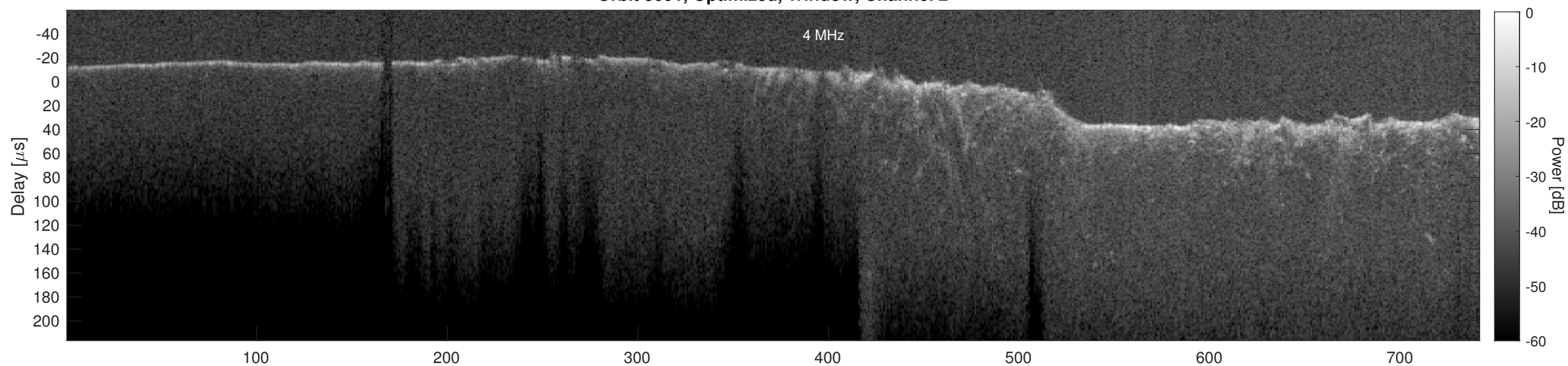
Orbit 3091, Cluttergram
