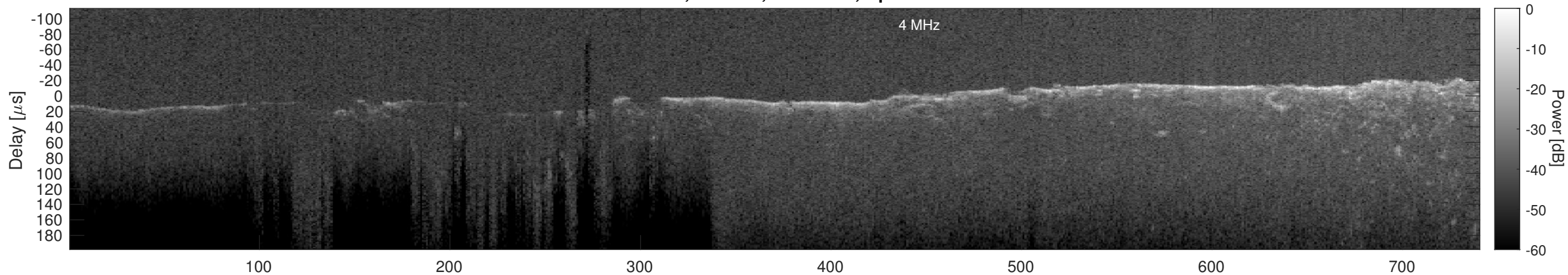
Orbit 3092, Cluttergram
