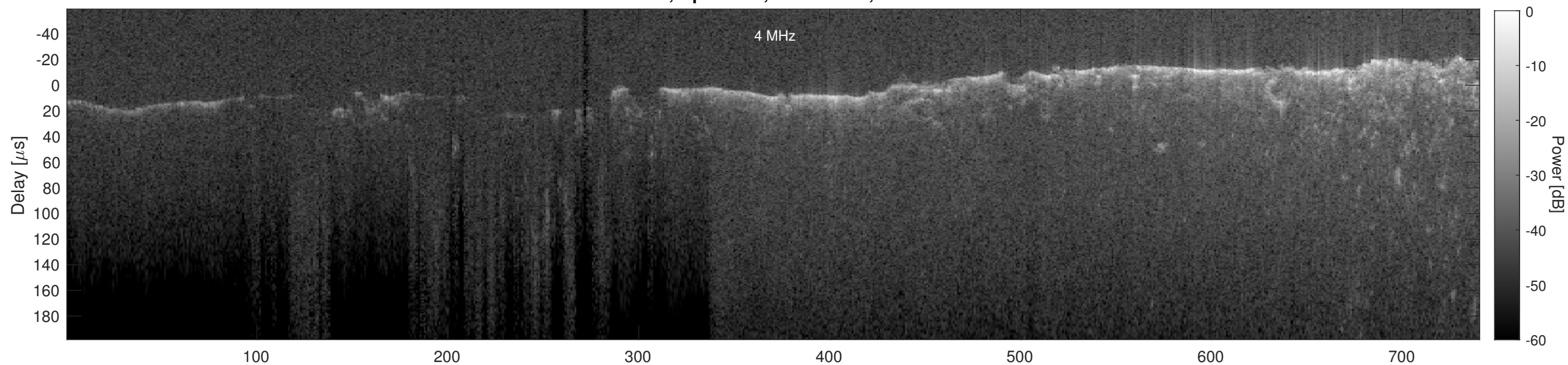
Orbit 3092, Cluttergram
