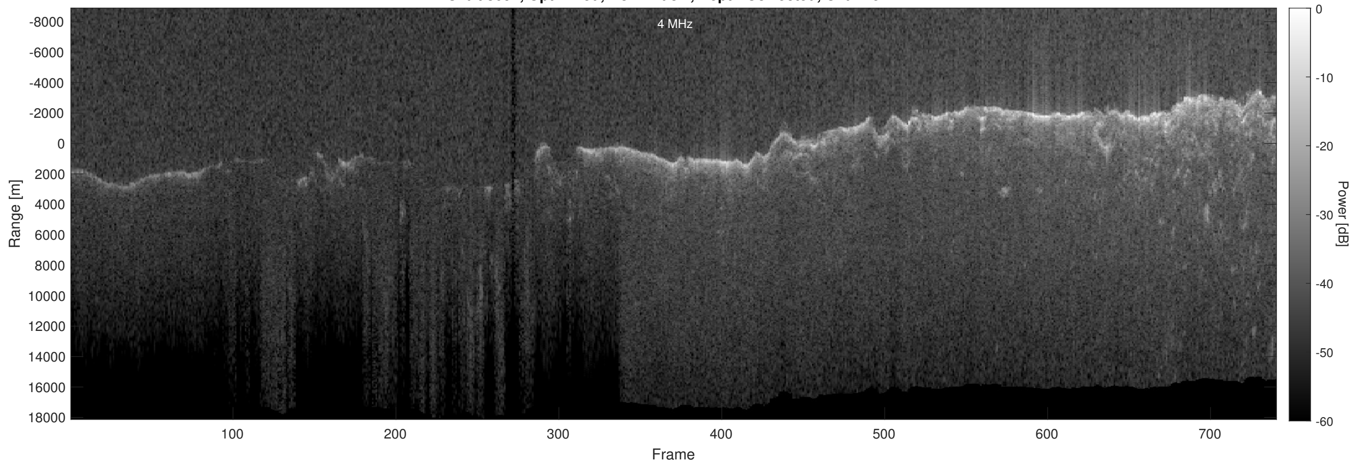
Orbit 3092, Optimized, No Window, Depth-Corrected, Channel 2
