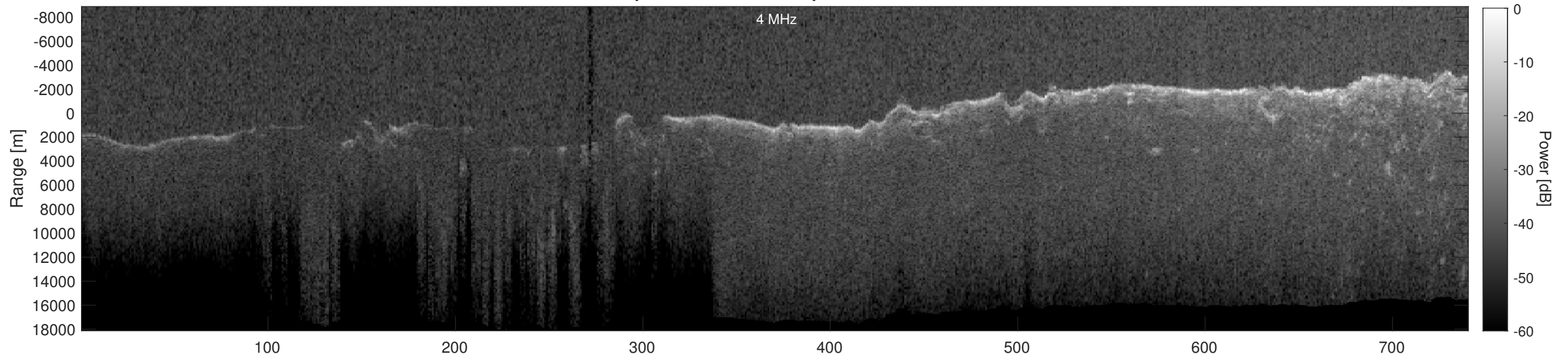
Orbit 3092, Depth-Corrected Cluttergram
