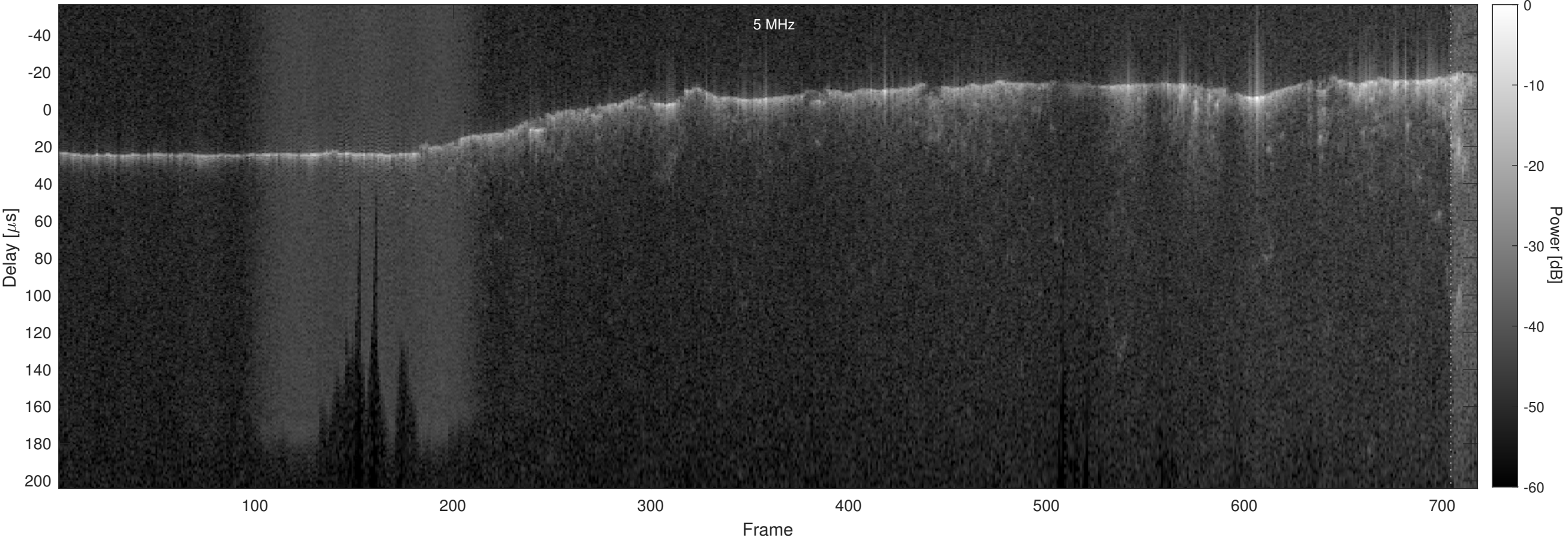
Orbit 3094, Optimized, No Window, Channel 2
